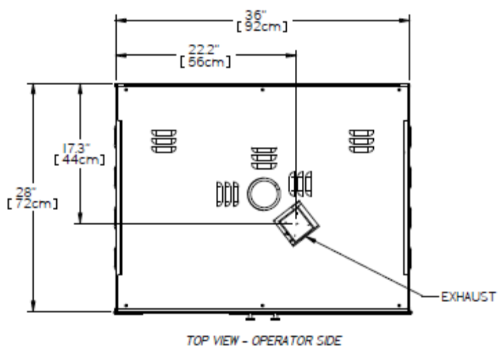
TOP VIEW - OPERATOR SIDE
